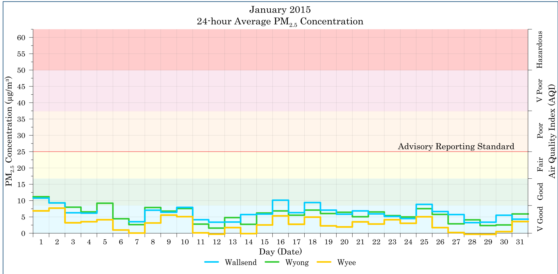
Figure 7-2: Lake Macquarie - Wyong 24-hour average PM 2.5 levels – January 2015
