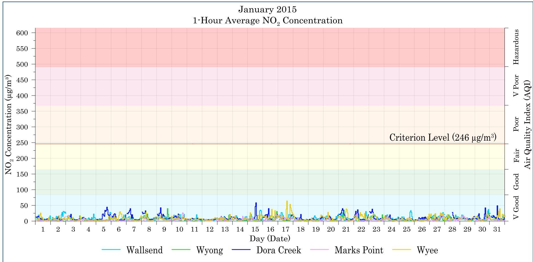
Figure 7-3: Lake Macquarie - Wyong 1-hour average NO 2 levels – January 2015
