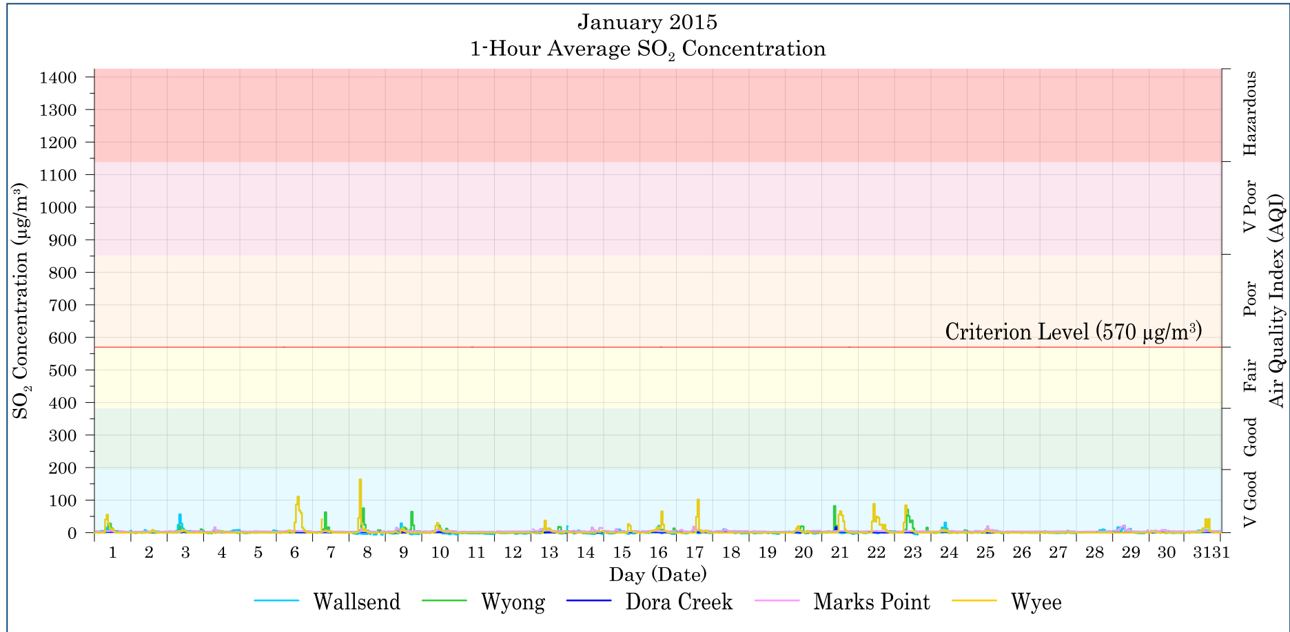
Figure 7-4: Lake Macquarie - Wyong 1-hour average SO 2 levels – January 2015
