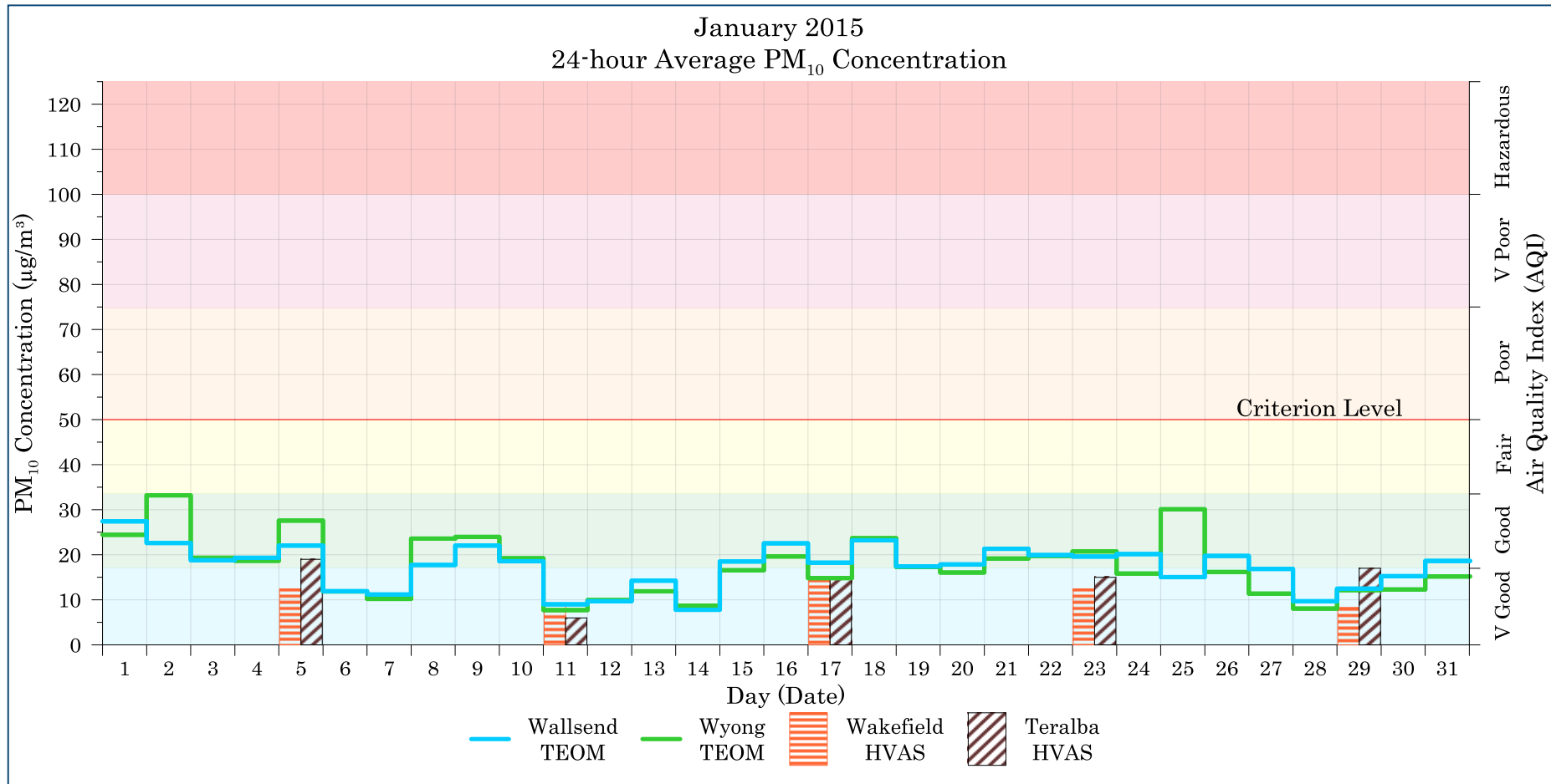
Figure 7-1: Lake Macquarie - Wyong 24-hour average PM 10 levels – January 2015
