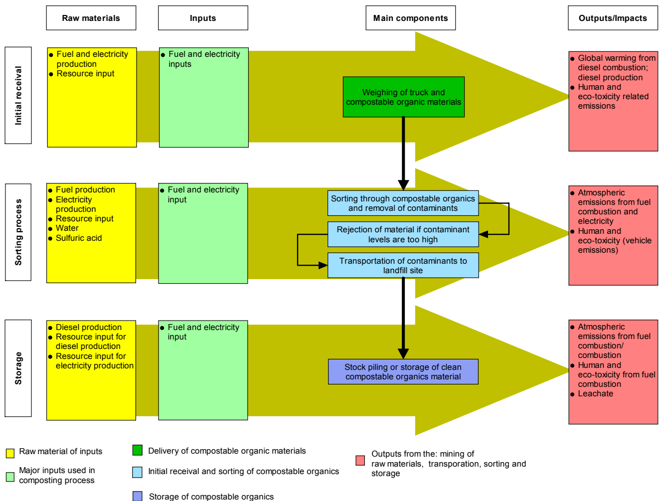
Figure 5.1 Sub-system model for compostable organic materials reveal process in windrow composting system model.
