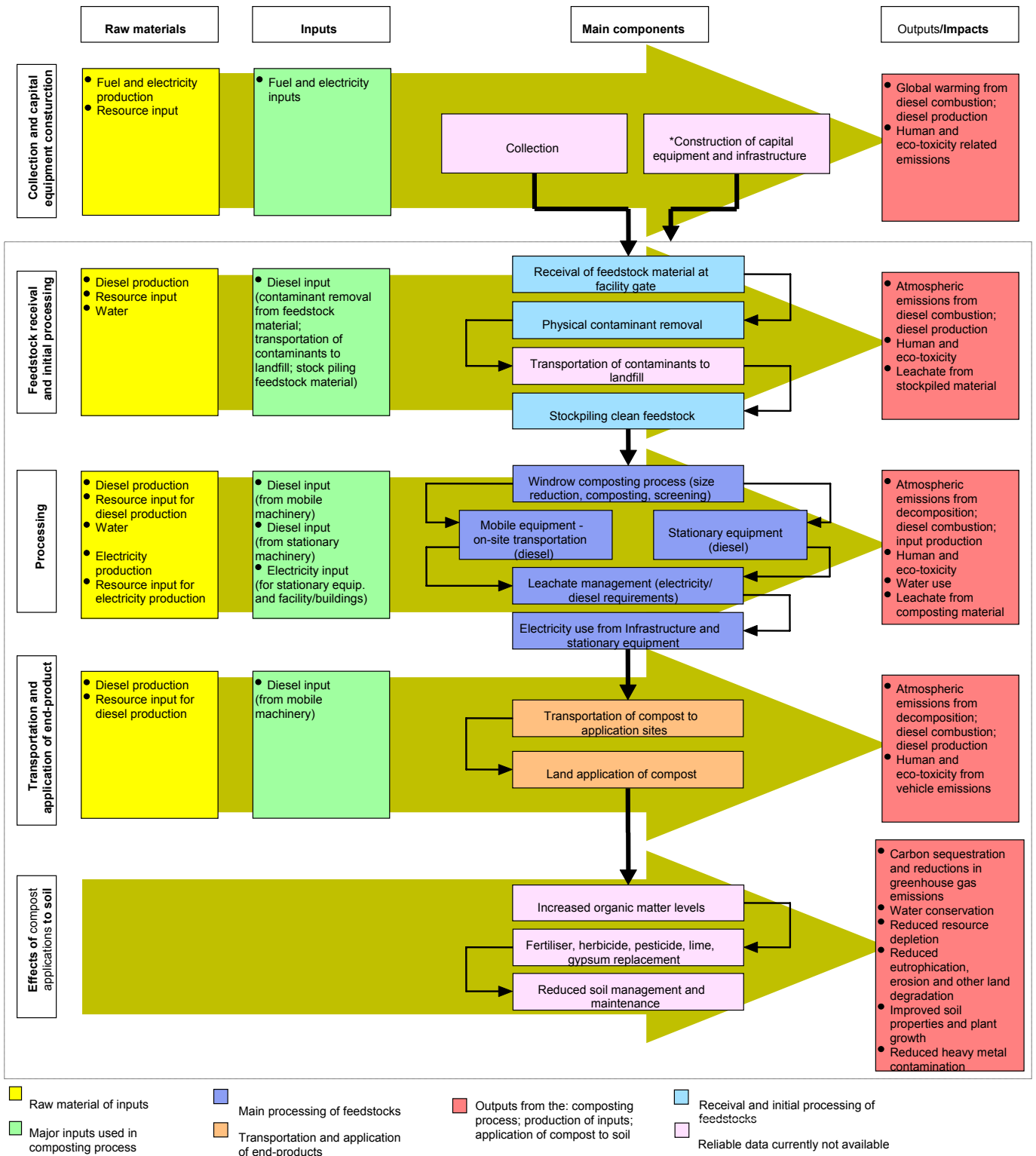
Figure 4.1 System model for windrow composting. * Note: environmental impacts from embodied energy in capital equipment and infrastructure are relevant to every stage of this model.
